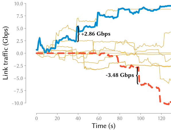
Figure 6: Load surges. The figure shows the link traffic over time of the 10 links with the largest load surges. The biggest positive (—) and negative (--) surges are also highlighted.
